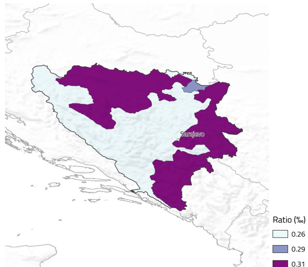
Regions of Highest Earthquake Risk
